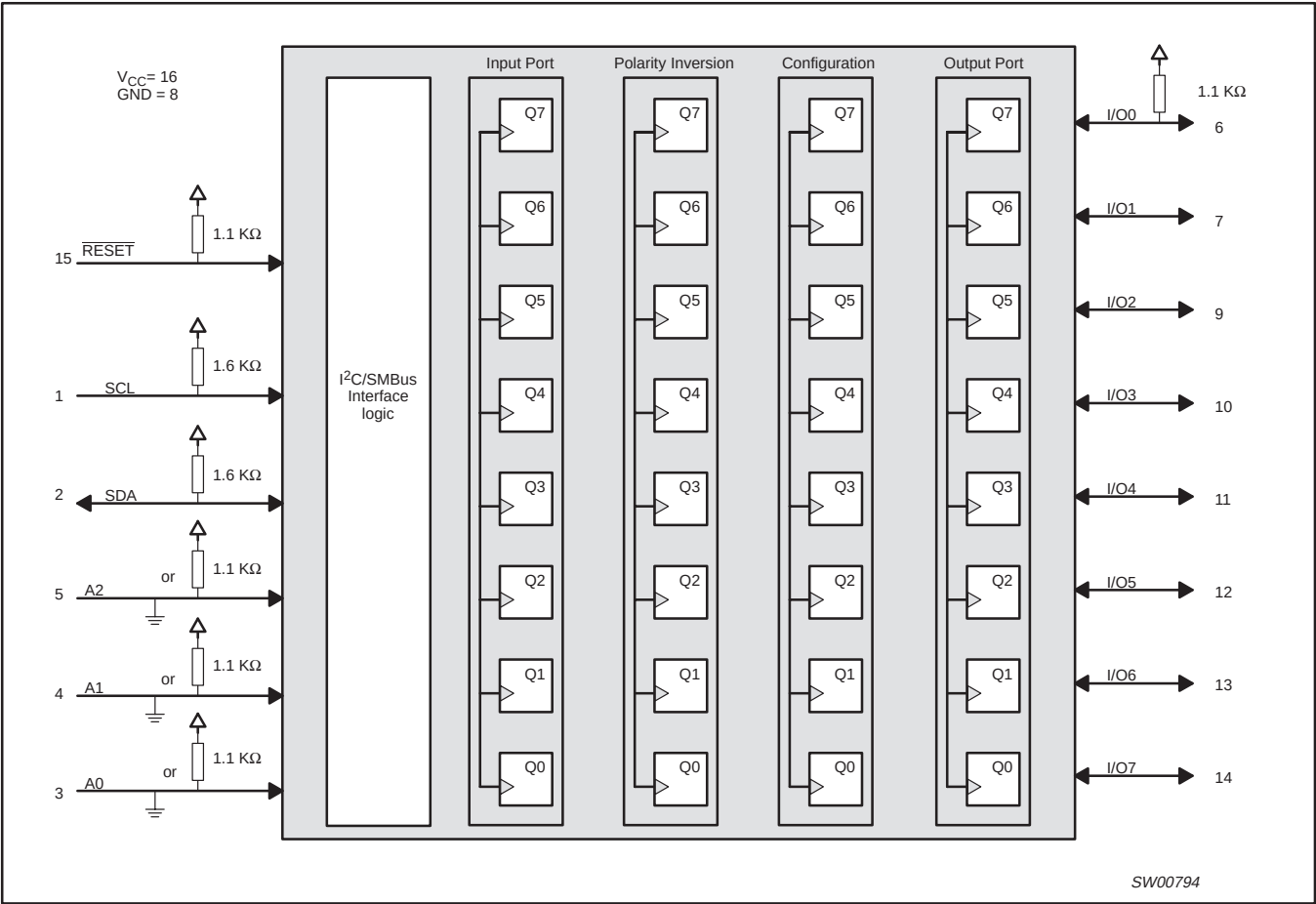
Figure 3. System diagram
